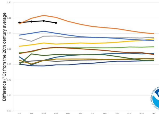
Year-to-date Global Temperatures for 2020 and the ten warmest years on record
