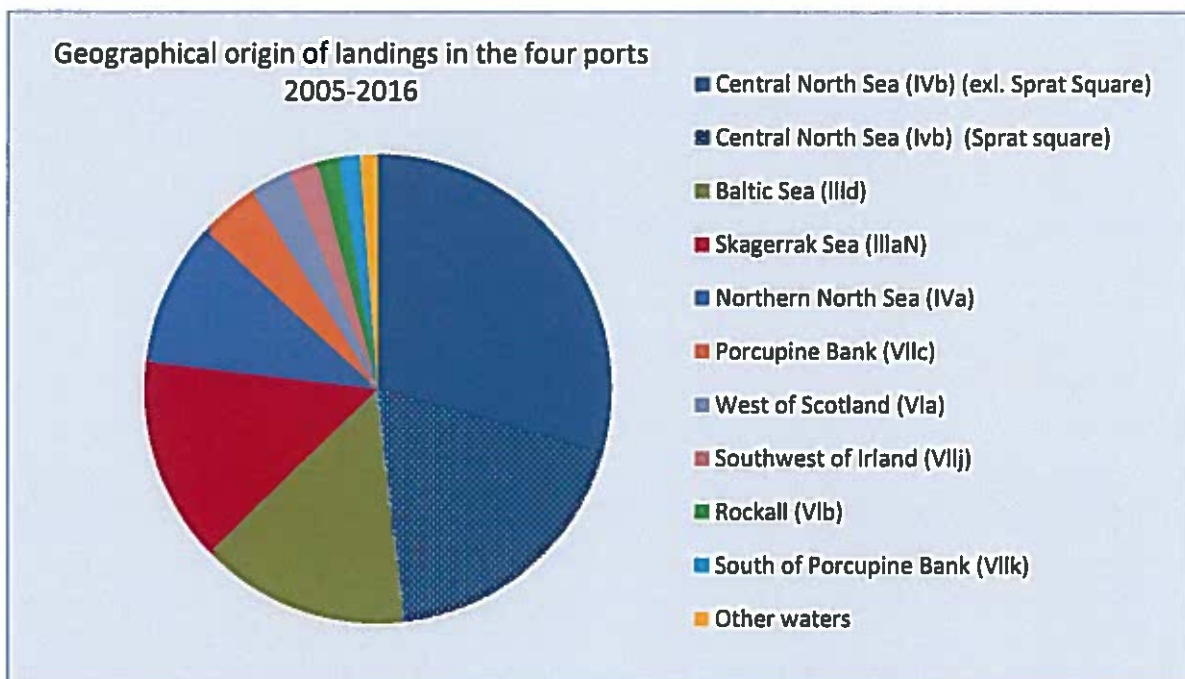
Figure 4.6: Catching area for landings in the four ports. ICES fishing areas, total 2005–2016. Other waters include: The sound (IIId), Western English Channel (VIIe), West of Ireland (VIIb) and Kattegat IIIaS. Source: The Ministry for Environment and Food, 2017. /LBST 2017, Dynamic landing statistics.
