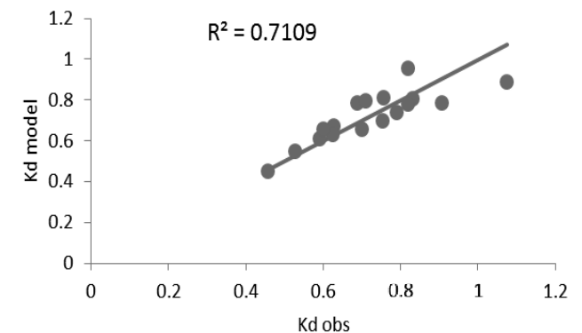
Scatterplot
