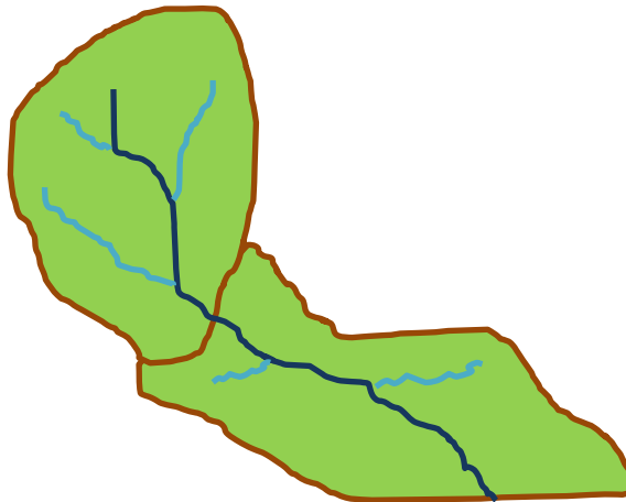
Figure 2. Sketch representing the stream flowing across several catchments (dark blue, “connect streams”) and stream flowing in only one catchment (light blue, “intern streams”).
