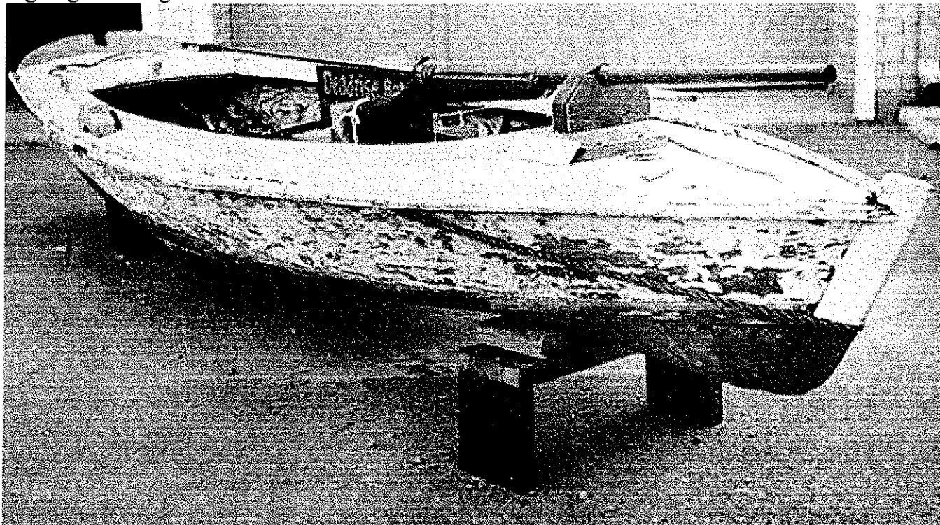
Big gun in deadrise skiff built by Ira Hudson, Chincoteague, Va., c. 1915.
