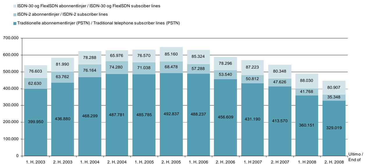
Figur 3. Abonnentlinjer hos anden operatør end TDC, 2003-2008 Figure 3. Subscriber lines with other operator than the incumbent, 2003-2008
