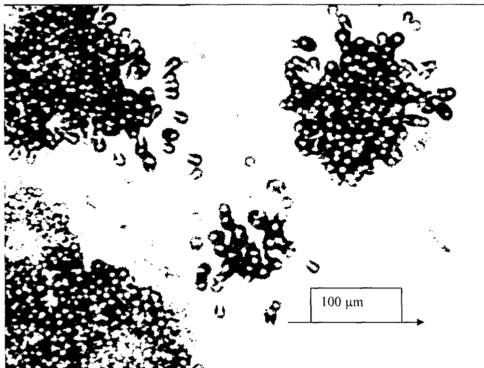
Fig. 6.1.5. CR-39 film exposed to a sediment sample showing tracks from alpha particles due to plutonium and americium.
