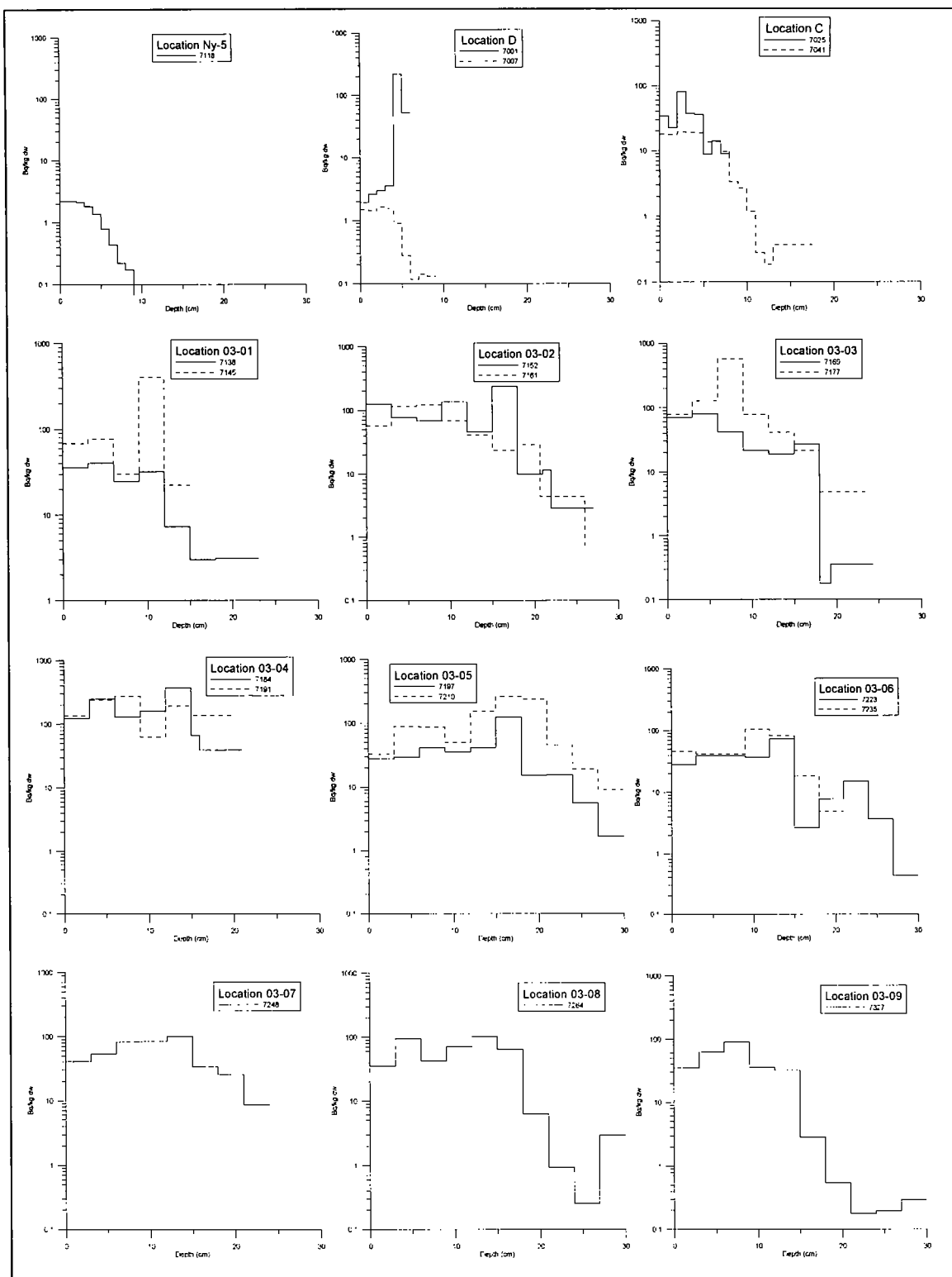
Fig. 6.1.1. Concentrations of ^{239,240}\text{Pu} in sediment cores from Bylot Sound ( \text{Bq kg}^{-1} dw).
