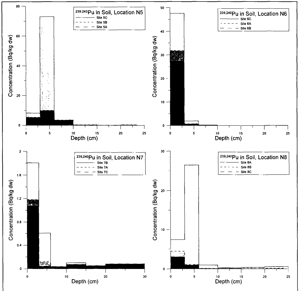
Fig. 6.6.2. Soil concentrations of ^{239,240}\text{Pu} ( \text{Bq kg}^{-1} \text{ dw} ) by depth at locations no. 5, 6, 7 and 8.
