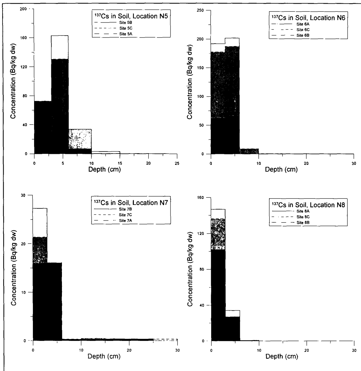
Fig. 6.6.6. Soil concentrations of 137 Cs (Bq kg -1 dw) by depth at locations no. 5, 6, 7 and 8.
