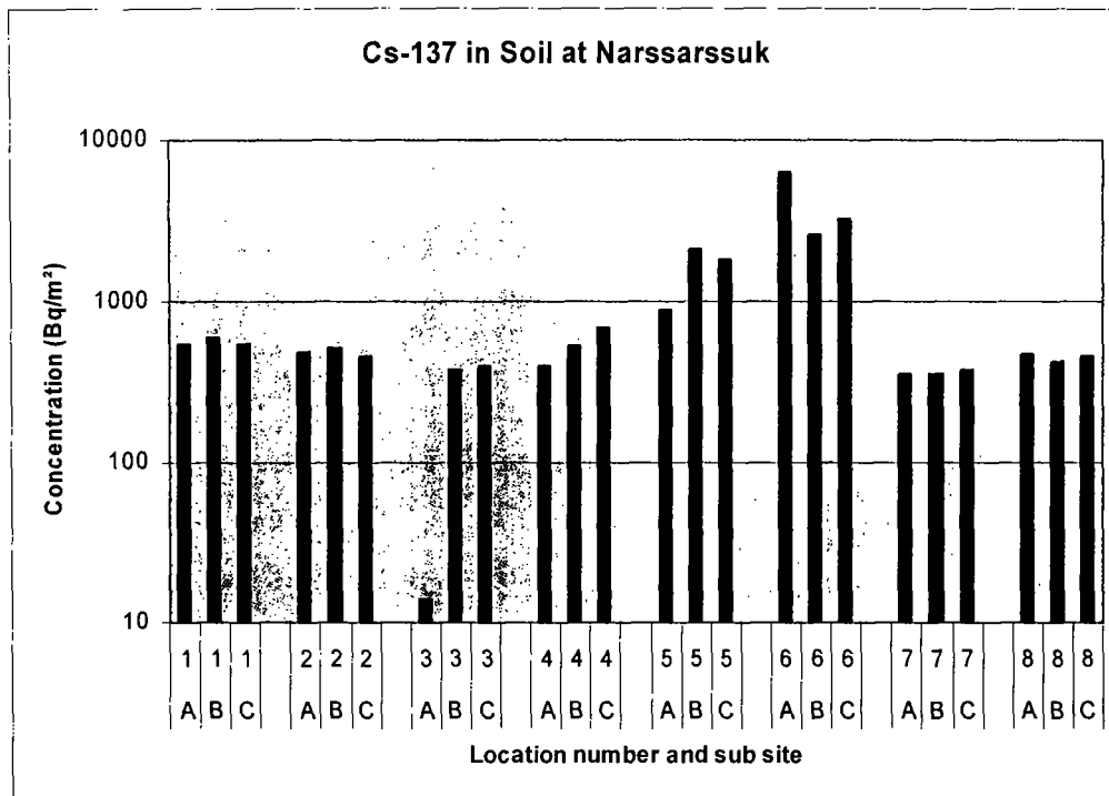
Fig. 6.6.7. Concentrations of 137 Cs (Bq m -2 ) in soil cores collected at Narssarsuk.
