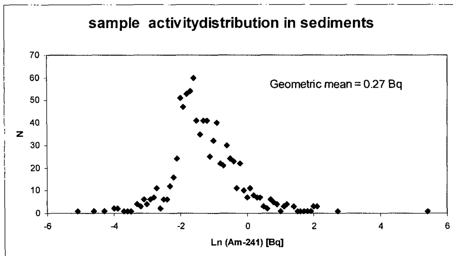
Fig. 6.1.4. Activity distribution of ^{241}\text{Am} in sediment samples.
