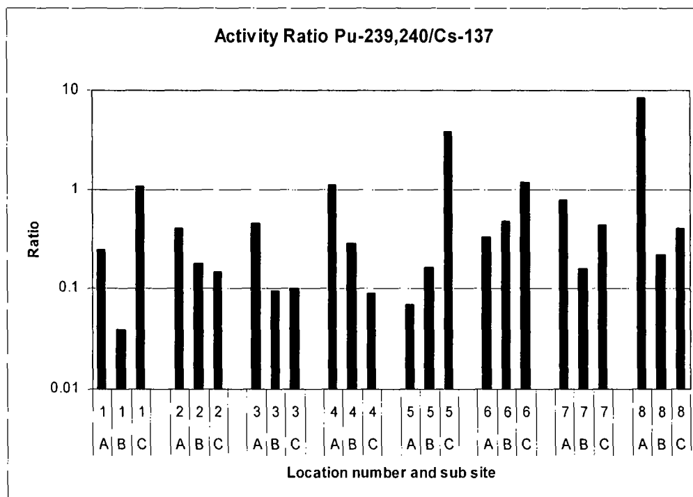
Fig. 6.6.8. Ratios of concentrations in soil of 239,240 Pu to those of 137 Cs (Bq m -2 per Bq m -2 ) across locations and sub sites at Narssarsuk.
