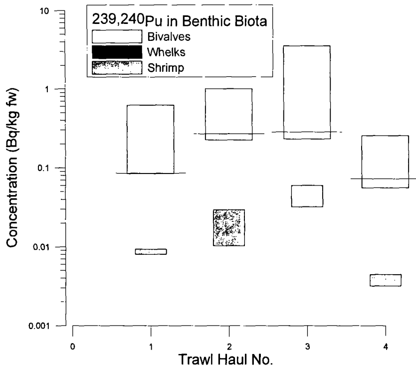
Fig. 6.4.1. Ranges of concentrations of ^{239,240}\text{Pu} in bivalves, whelks and shrimp.
